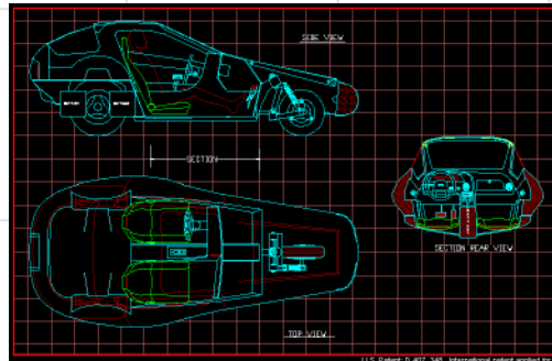
Project 32 tilting three-wheel vehicle designed for Transit Innovations, Fairfax, Virginia.
